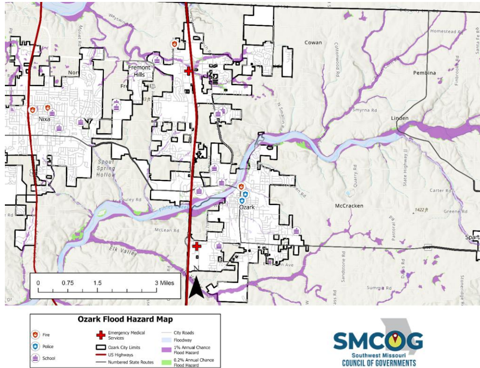
Figure 3.8. Ozark SFHA
